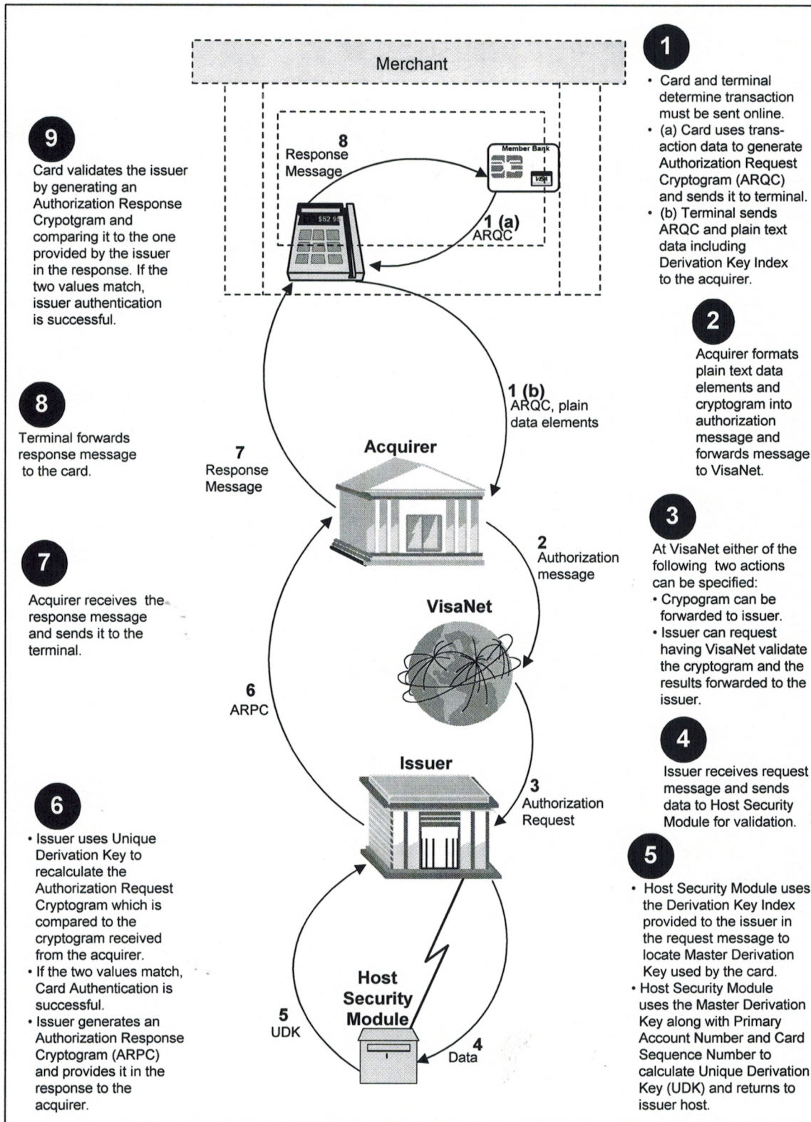
Figure 6-5: Role of DES Keys in Transaction Processing
